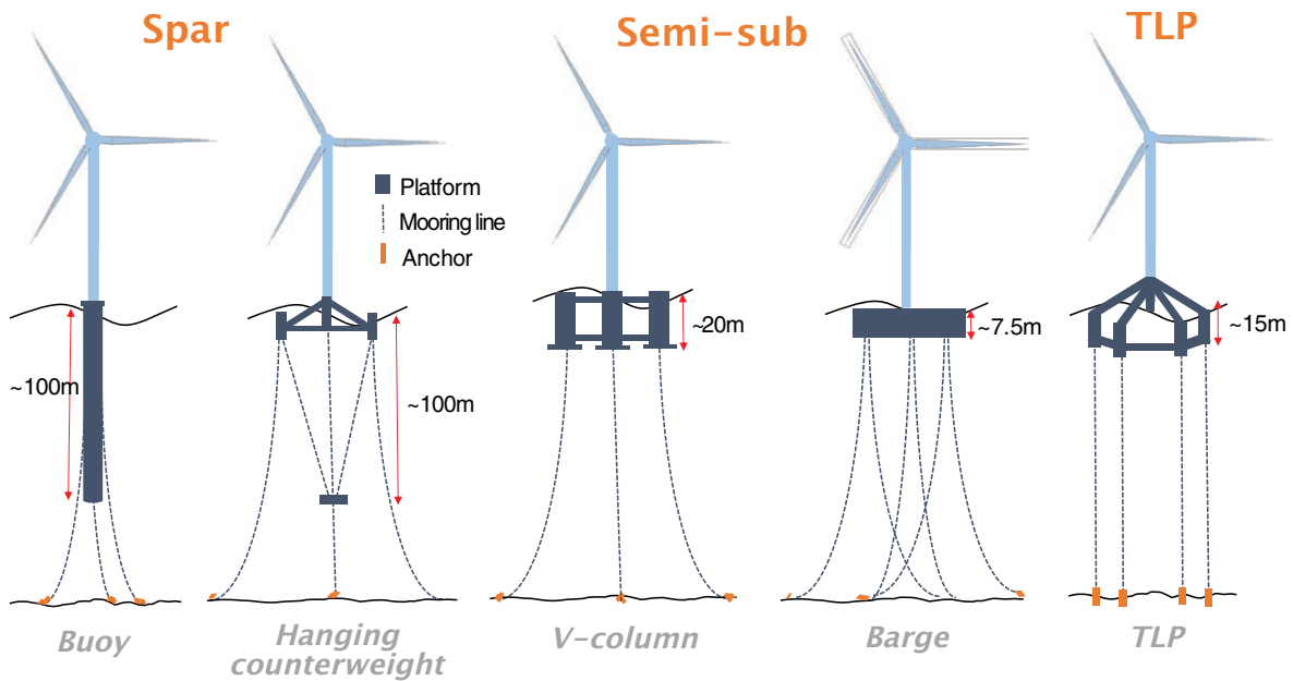
FIGURE 4: EXAMPLE FLOATING OFFSHORE WIND DESIGNS
