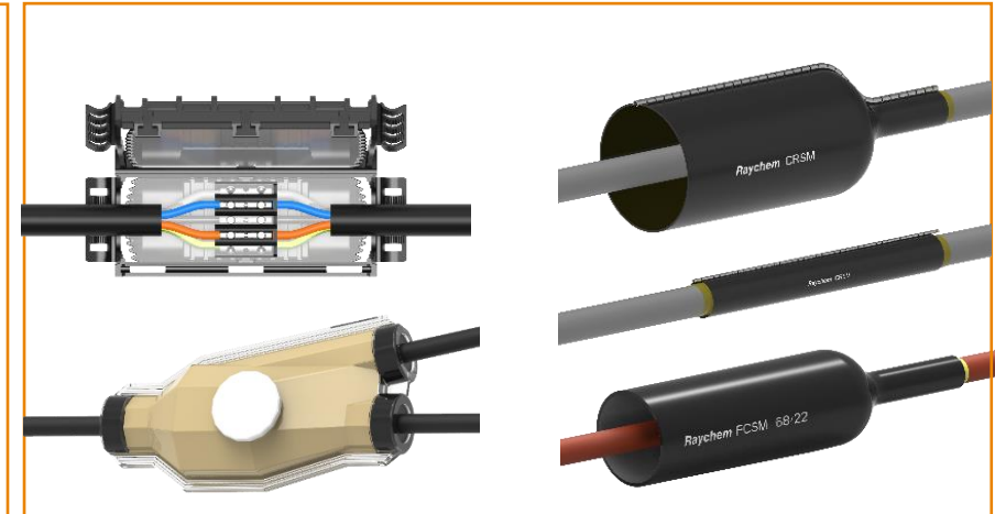
Heat Shrink and Cold Applied Components
